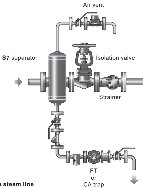
Fig. 8 Separator on a steam line
