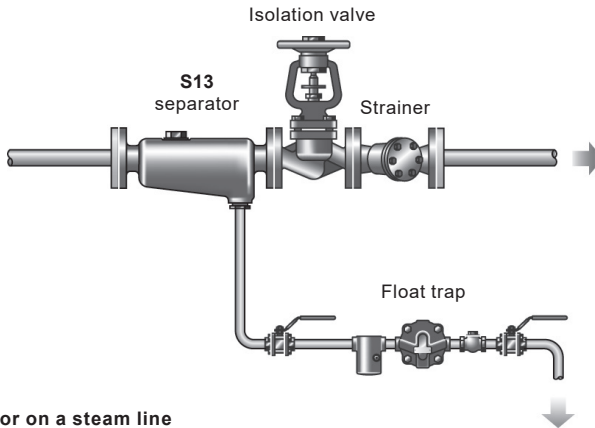
Fig. 6 Separator on a steam line
